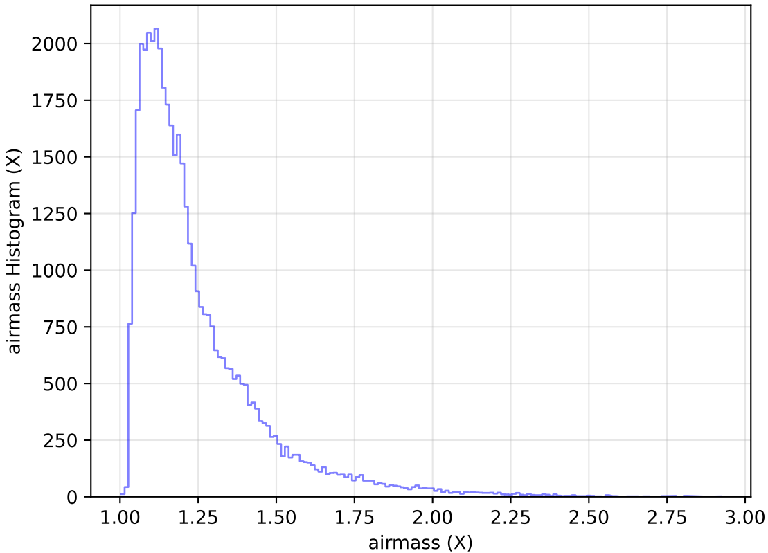
roll_pause_mjdp180_v3.4_10yrs Yr 1 y band: airmass Histogram
