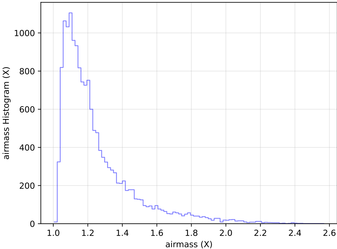
roll_pause_mjdp180_v3.4_10yrs Yr 1 u band: airmass Histogram
