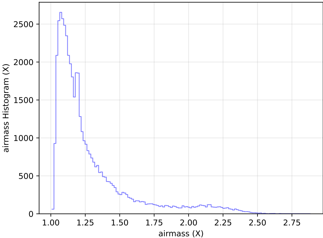
roll_pause_mjdp180_v3.4_10yrs Yr 1 r band: airmass Histogram
