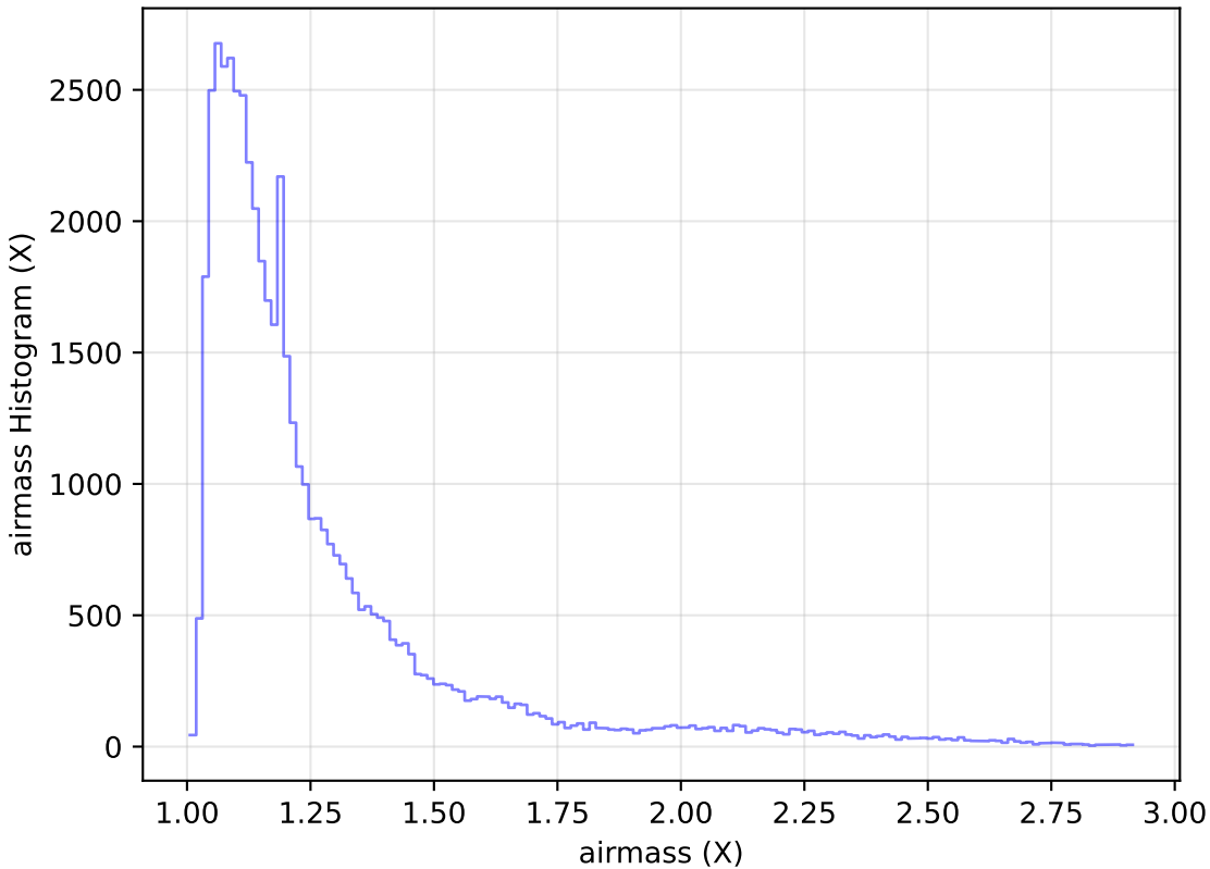
roll_pause_mjdp180_v3.4_10yrs Yr 1 i band: airmass Histogram
