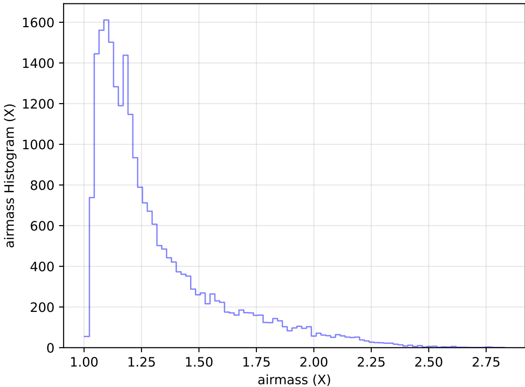
roll_pause_mjdp180_v3.4_10yrs Yr 1 g band: airmass Histogram
