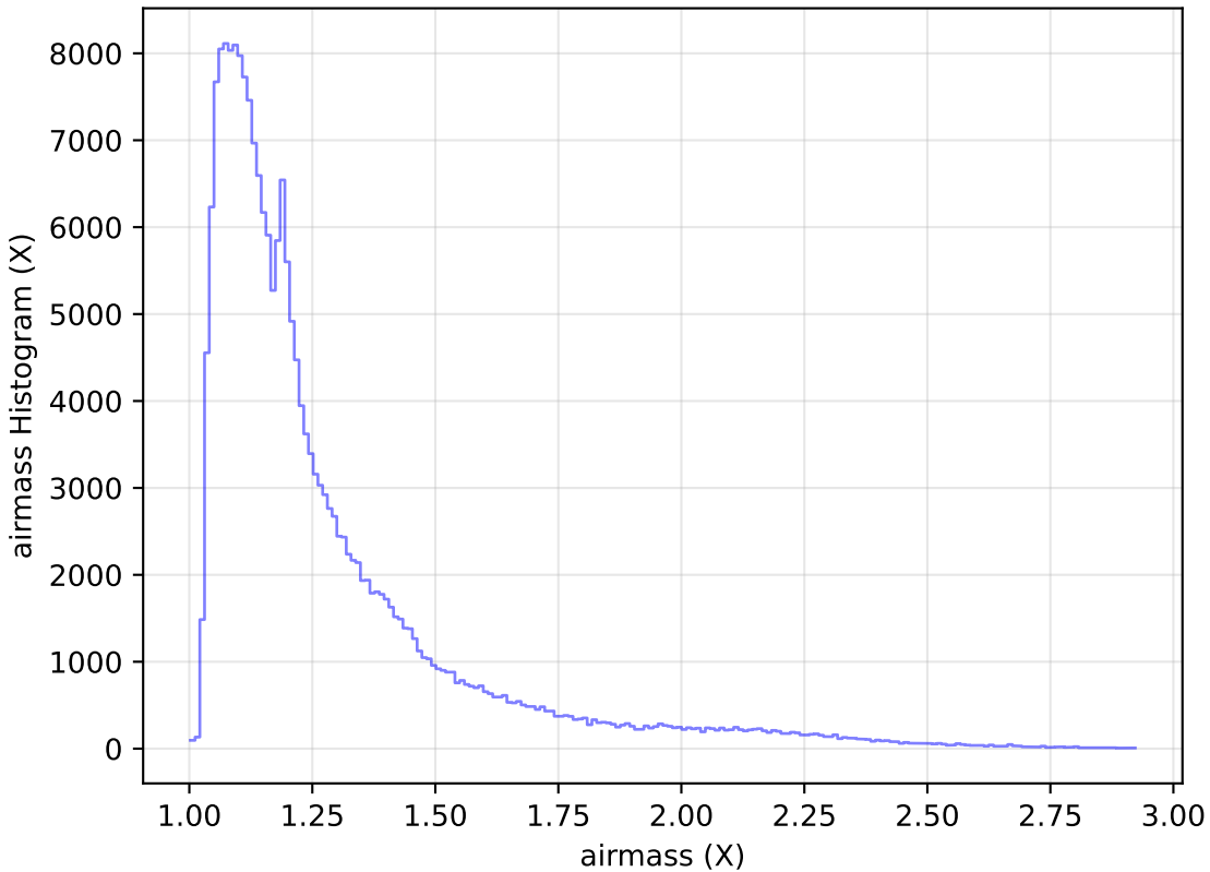
roll_pause_mjdp180_v3.4_10yrs Yr 1 all bands: airmass Histogram
