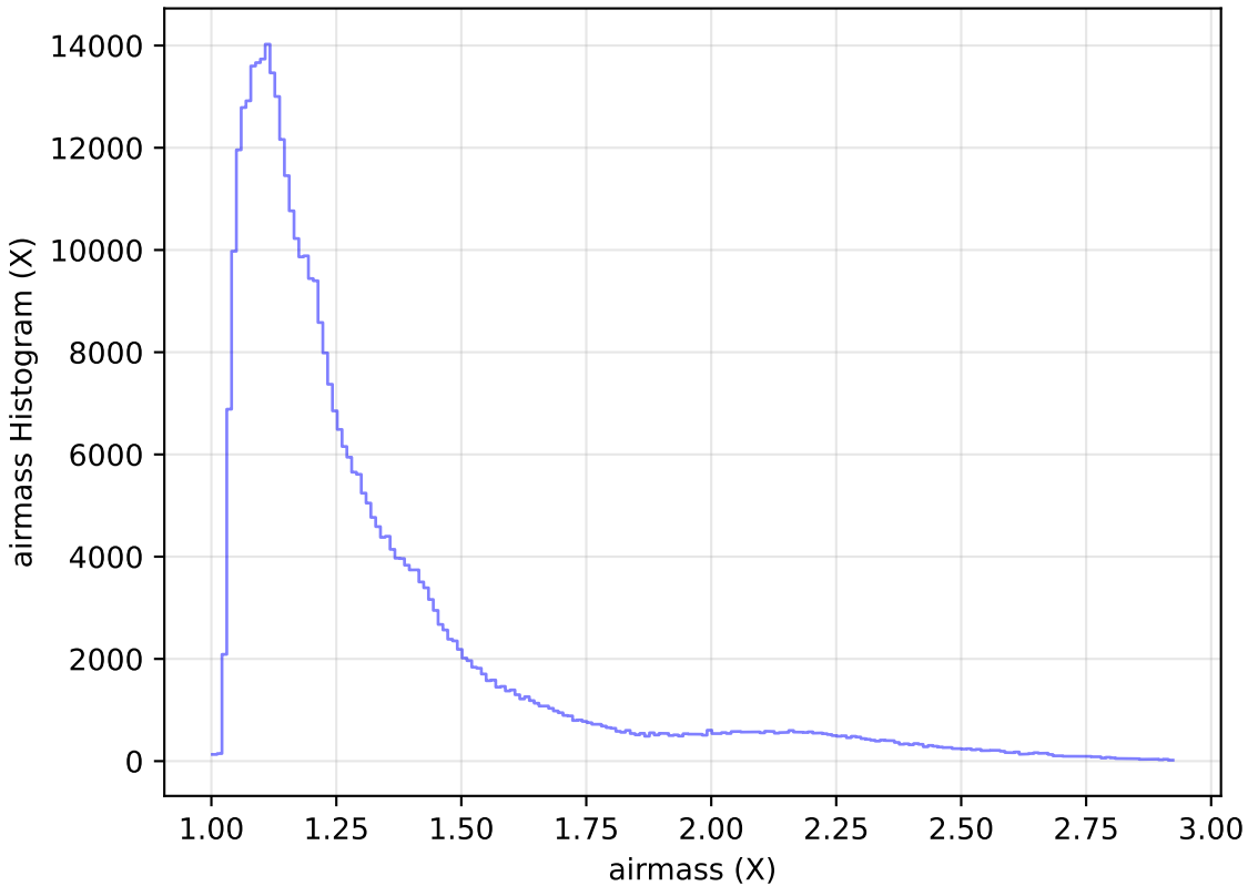
roll_pause_mjdp180_v3.4_10yrs WFD z band: airmass Histogram
