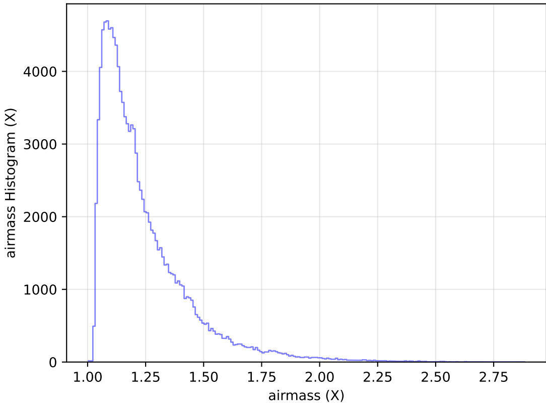
roll_pause_mjdp180_v3.4_10yrs WFD u band: airmass Histogram
