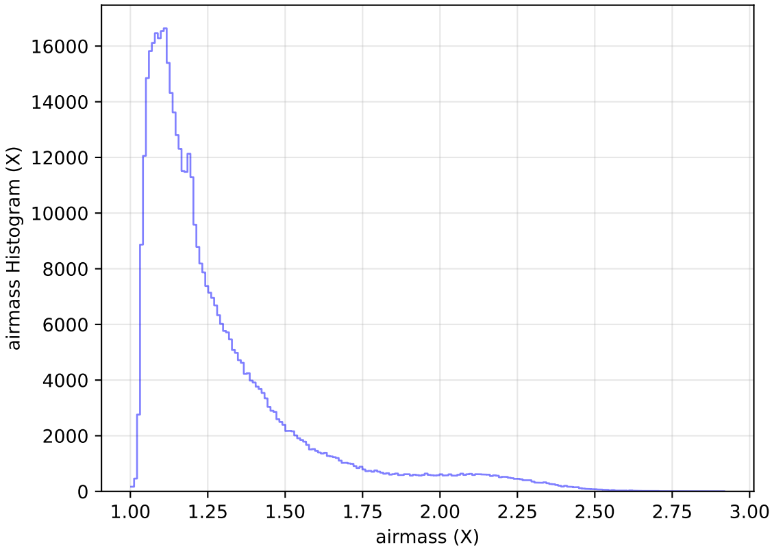
roll_pause_mjdp180_v3.4_10yrs WFD r band: airmass Histogram
