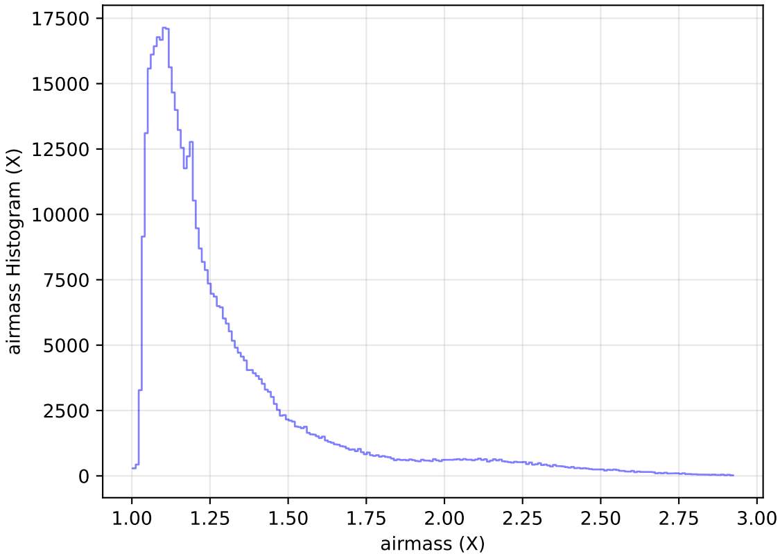
roll_pause_mjdp180_v3.4_10yrs WFD i band: airmass Histogram
