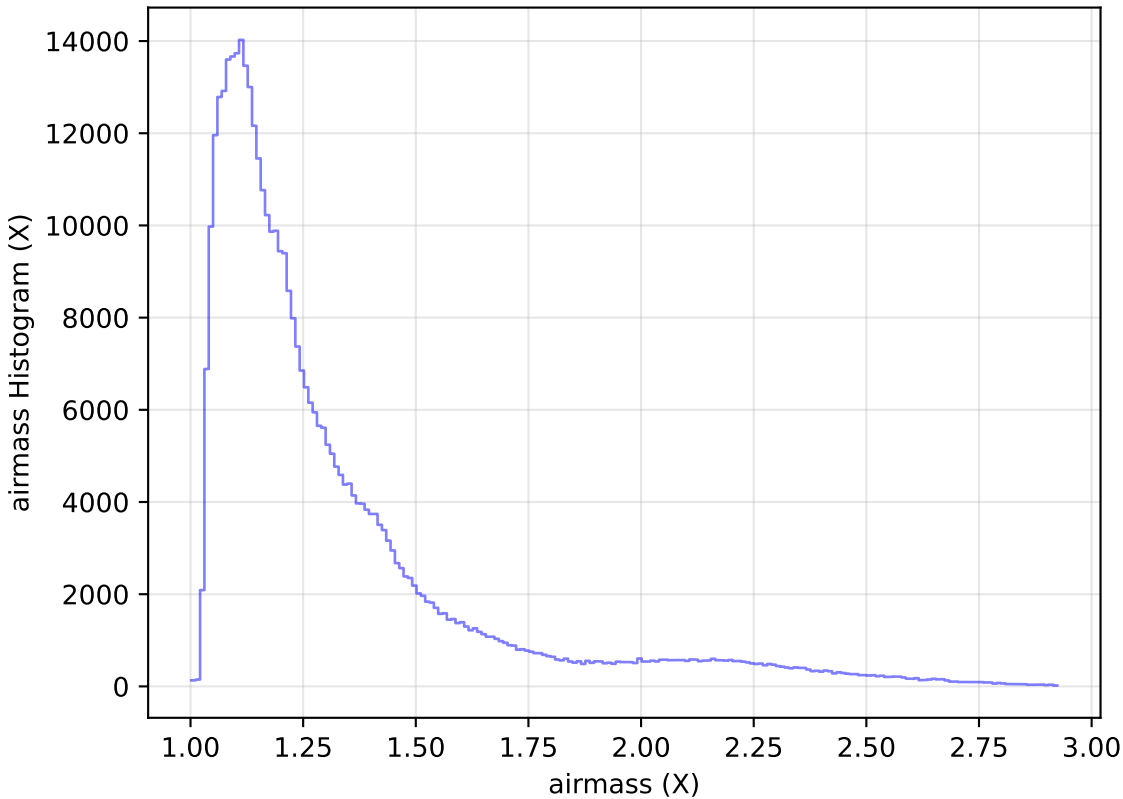
roll_pause_mjdp180_v3.4_10yrs All sky z band: airmass Histogram
