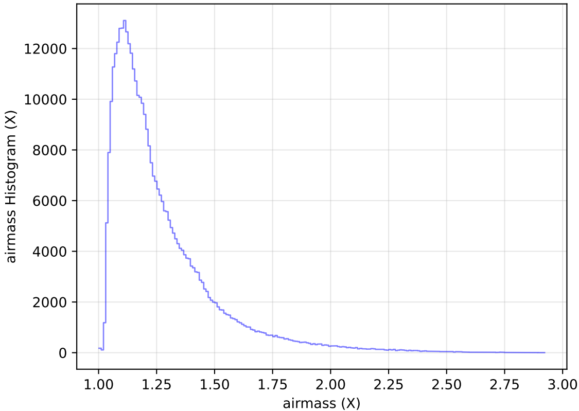
roll_pause_mjdp180_v3.4_10yrs All sky y band: airmass Histogram
