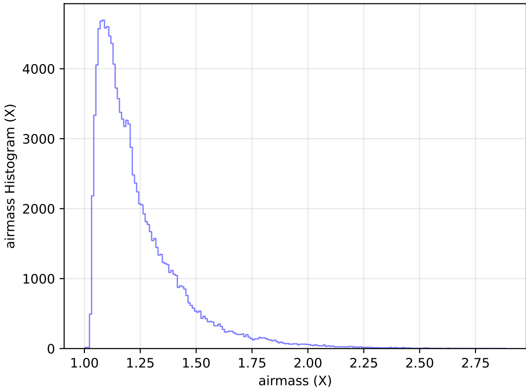
roll_pause_mjdp180_v3.4_10yrs All sky u band: airmass Histogram
