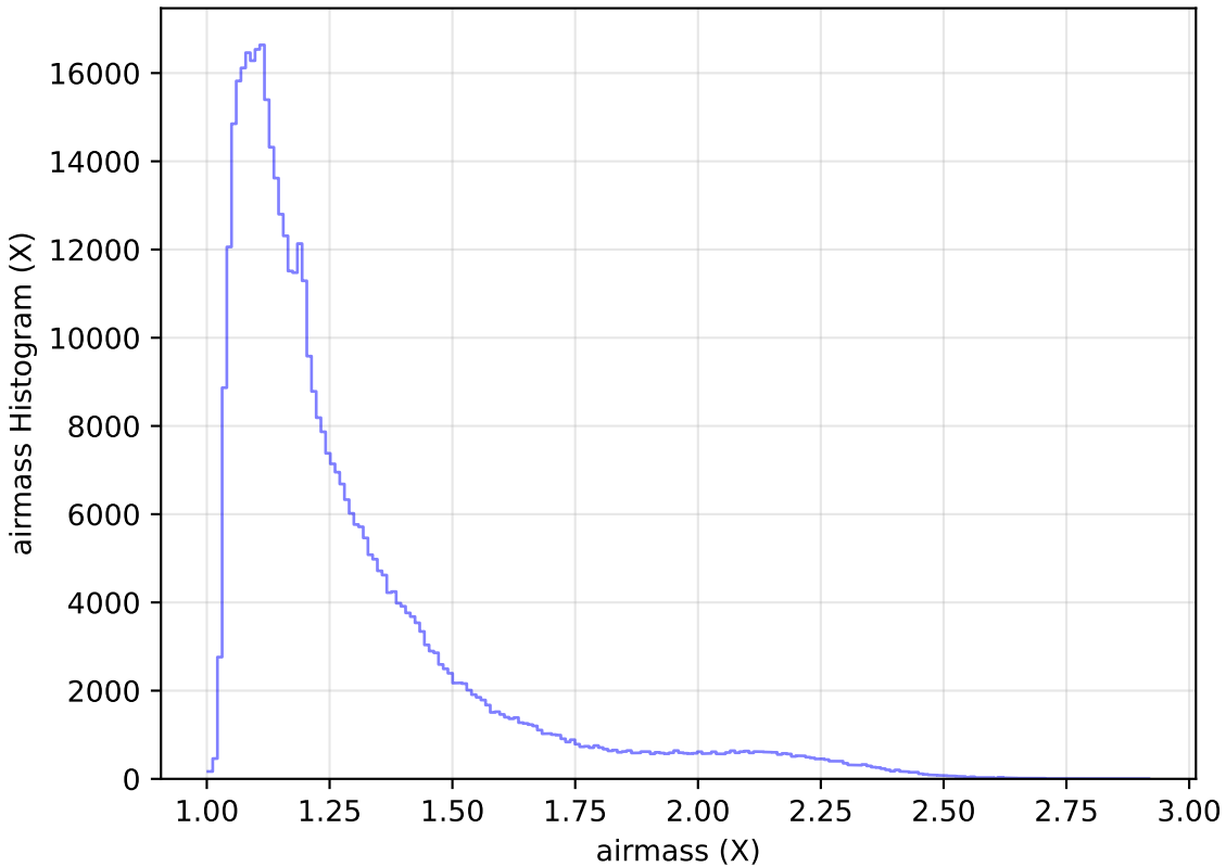
roll_pause_mjdp180_v3.4_10yrs All sky r band: airmass Histogram
