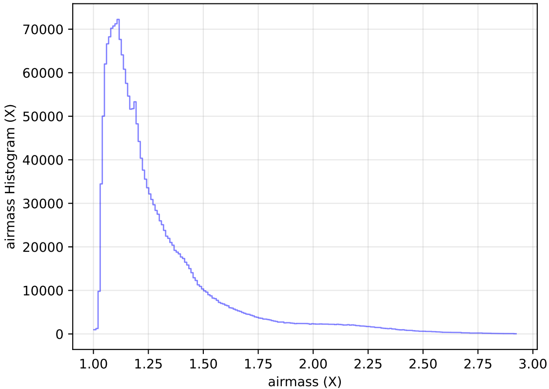
roll_pause_mjdp180_v3.4_10yrs All sky all bands: airmass Histogram
