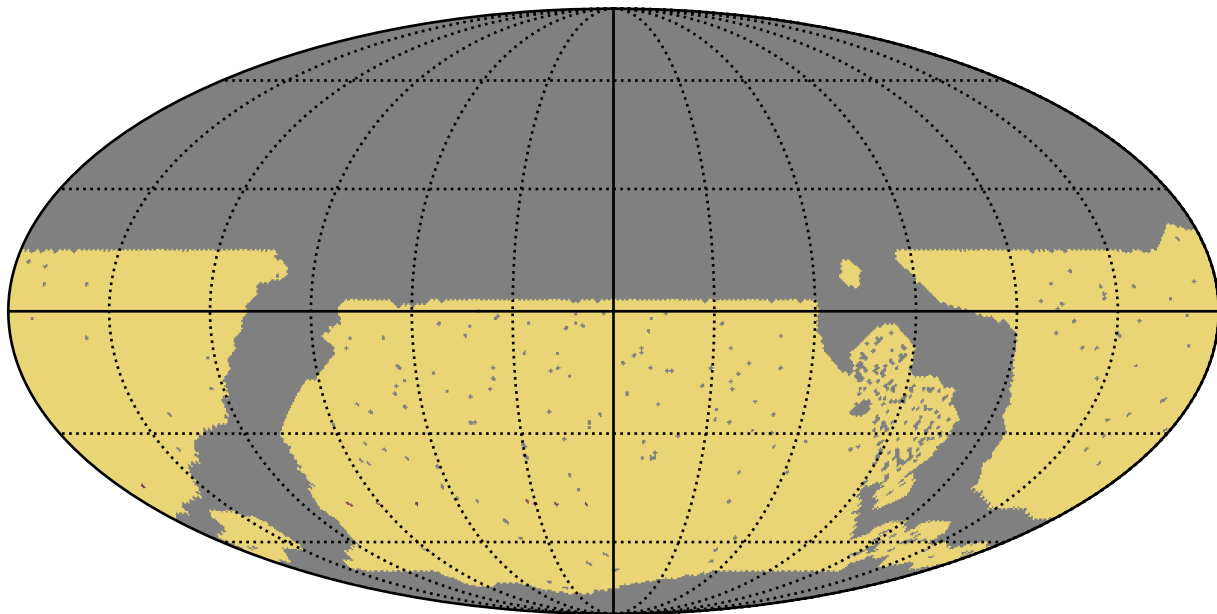
roll_pause_mjdp180_v3.4_10yrs WFD: RapidRevisits
