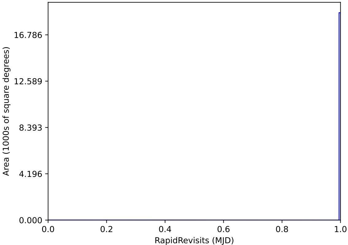
roll_pause_mjdp180_v3.4_10yrs WFD: RapidRevisits
