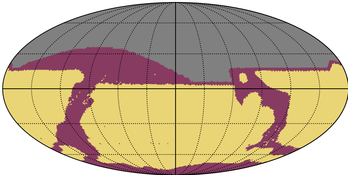
roll_pause_mjdp180_v3.4_10yrs All sky: RapidRevisits
