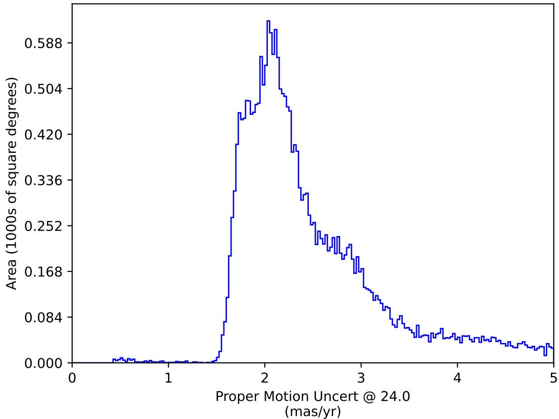
roll_pause_mjdp180_v3.4_10yrs All sky: Proper Motion Uncert @ 24.0
