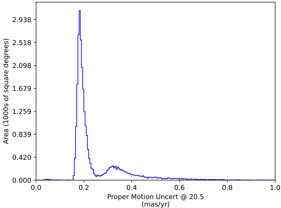
roll_pause_mjdp180_v3.4_10yrs All sky: Proper Motion Uncert @ 20.5
