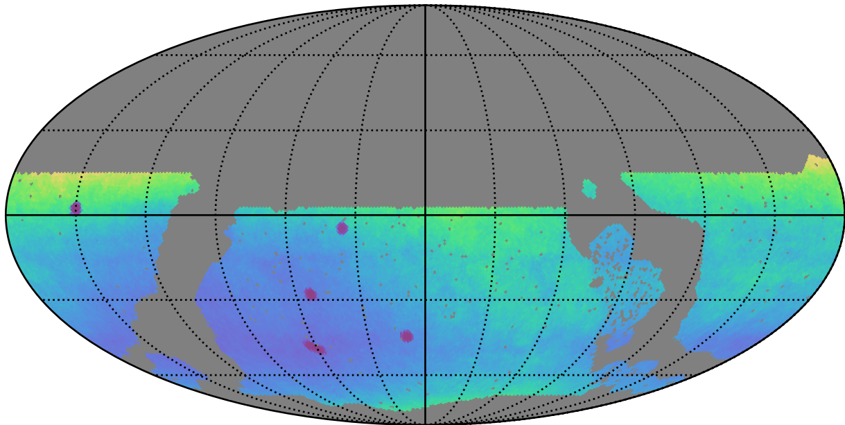
roll_pause_mjdp180_v3.4_10yrs WFD: Parallax Uncert @ 24.0
