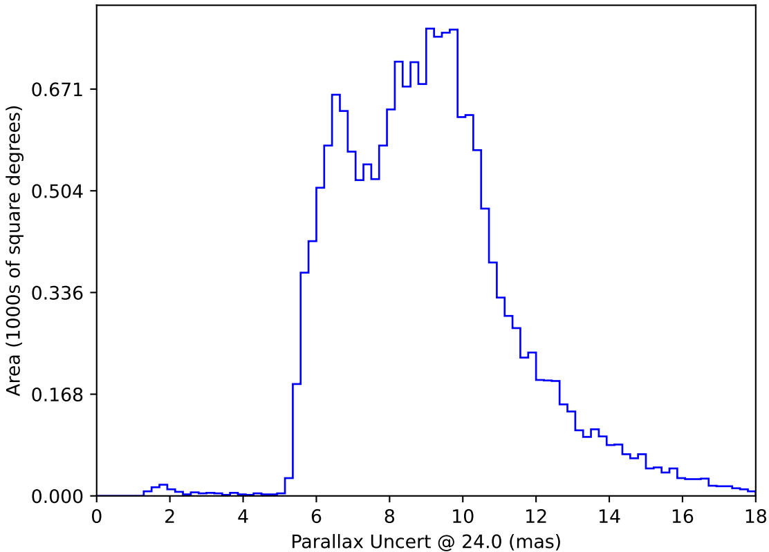
roll_pause_mjdp180_v3.4_10yrs WFD: Parallax Uncert @ 24.0
