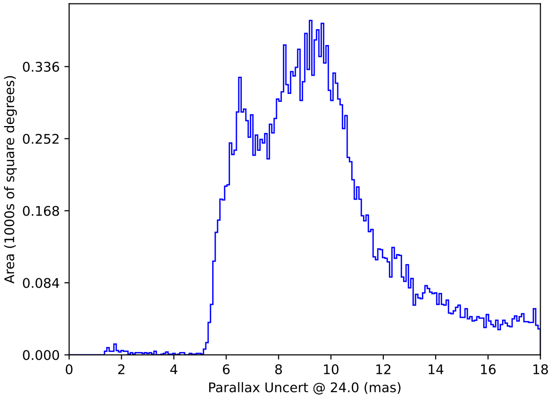
roll_pause_mjdp180_v3.4_10yrs All sky: Parallax Uncert @ 24.0
