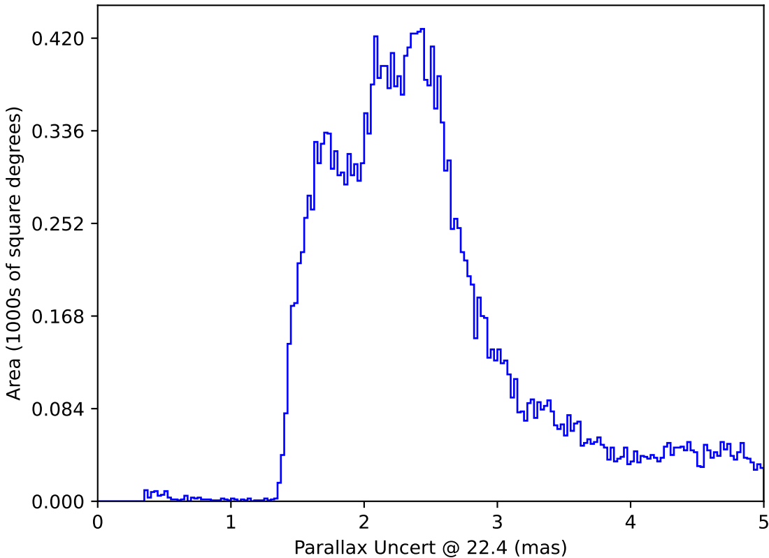
roll_pause_mjdp180_v3.4_10yrs All sky: Parallax Uncert @ 22.4
