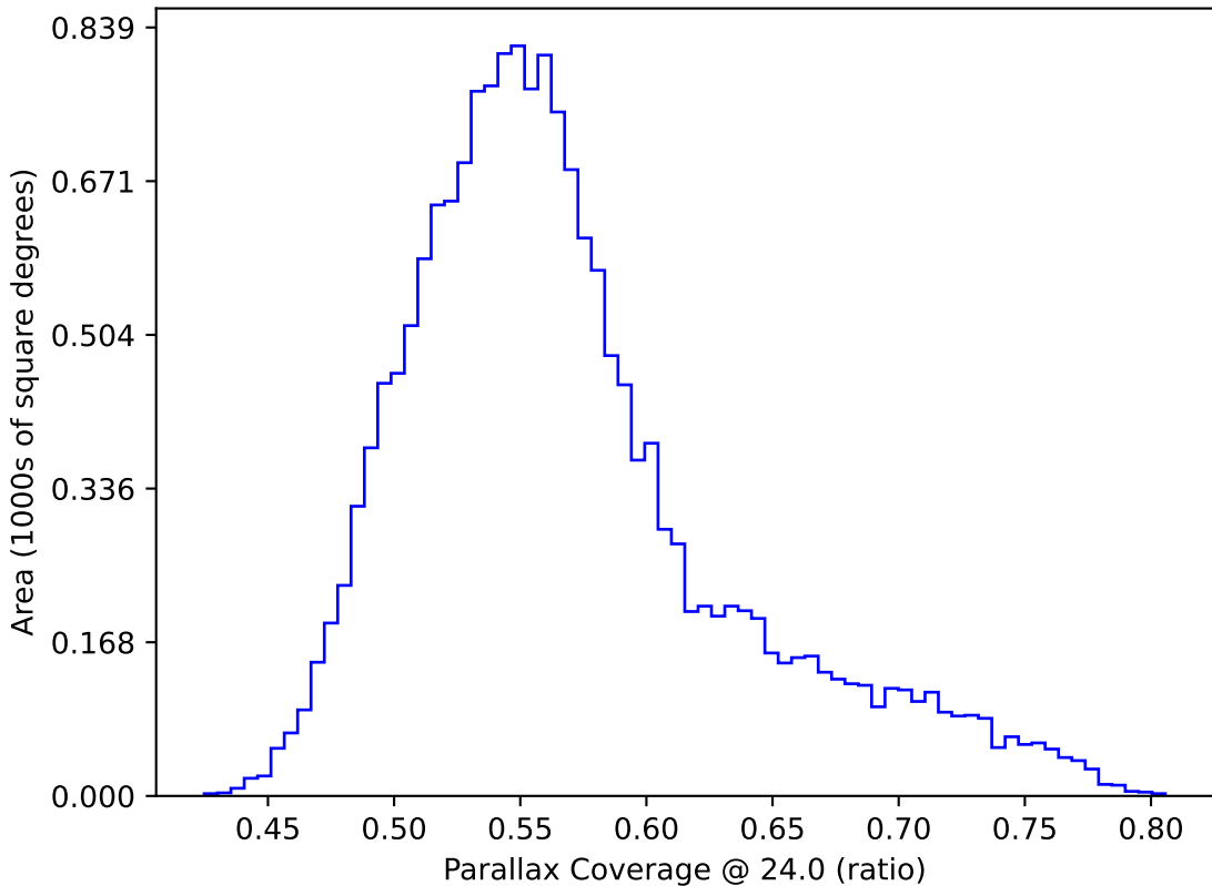
roll_pause_mjdp180_v3.4_10yrs WFD: Parallax Coverage @ 24.0
