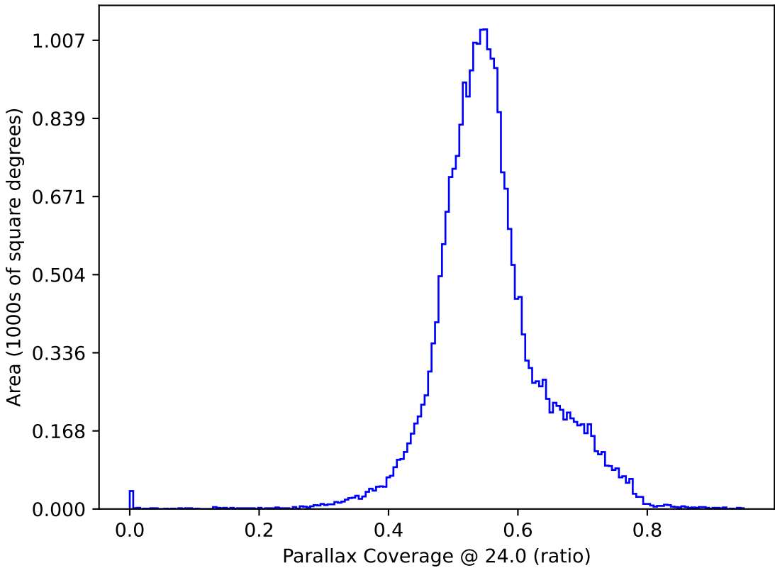
roll_pause_mjdp180_v3.4_10yrs All sky: Parallax Coverage @ 24.0
