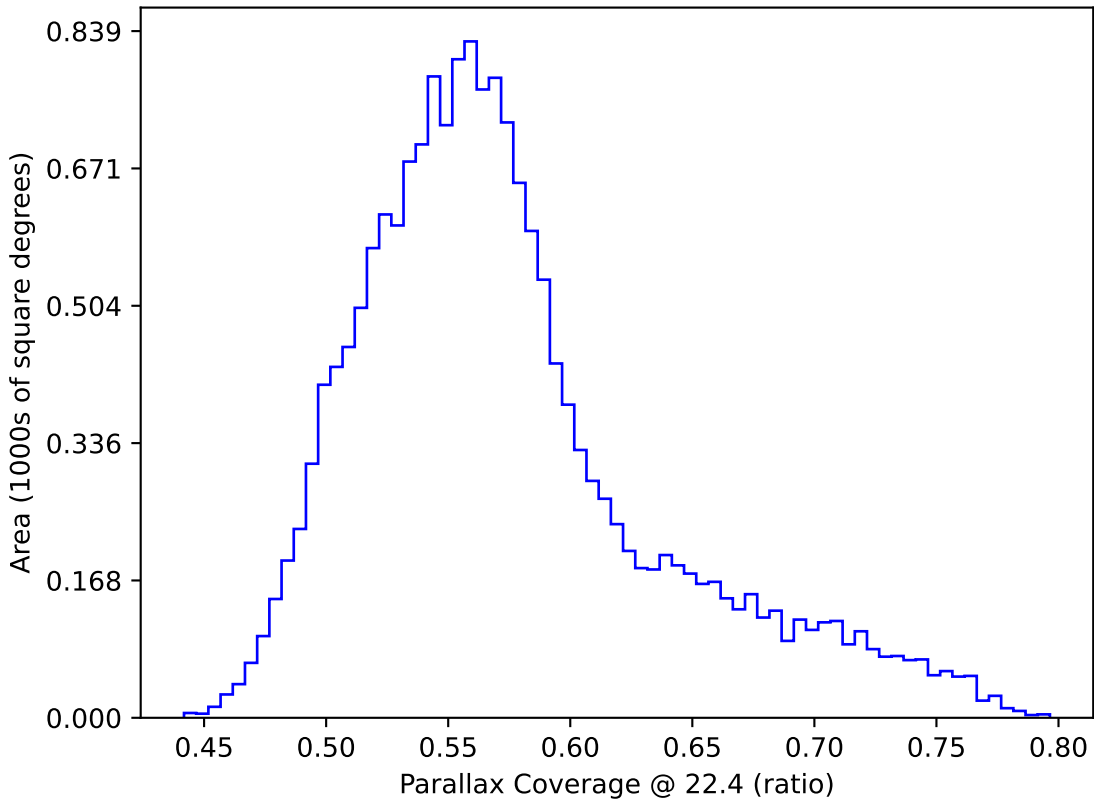
roll_pause_mjdp180_v3.4_10yrs WFD: Parallax Coverage @ 22.4
