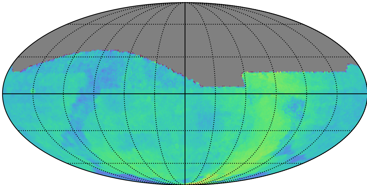
roll_pause_mjdp180_v3.4_10yrs All sky: Parallax Coverage @ 22.4
