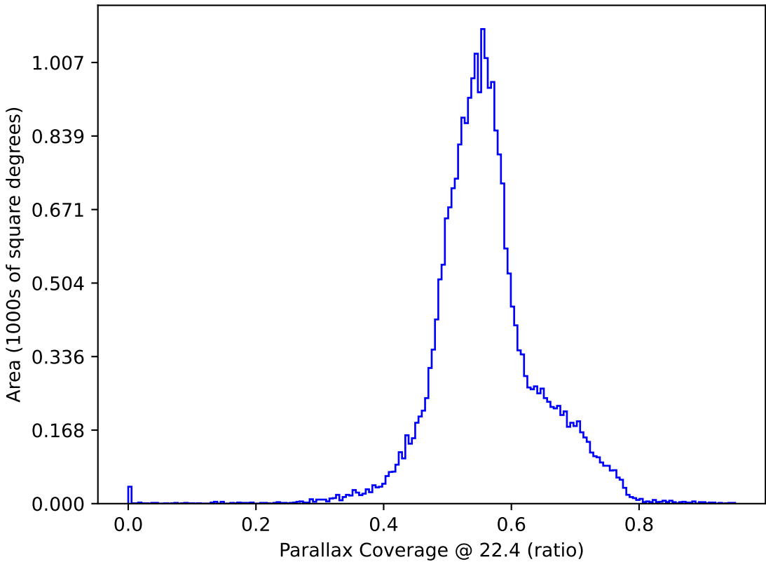
roll_pause_mjdp180_v3.4_10yrs All sky: Parallax Coverage @ 22.4
