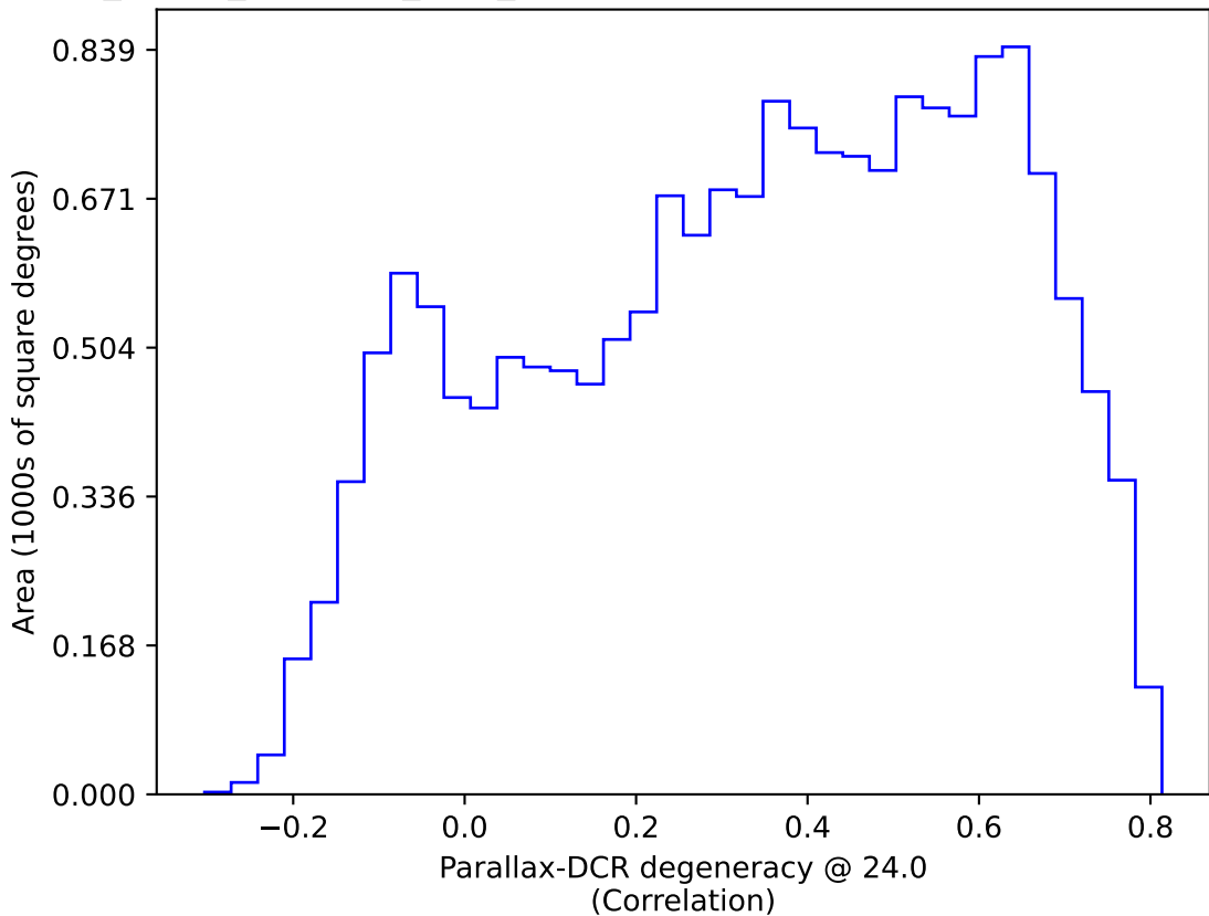
roll_pause_mjdp180_v3.4_10yrs WFD: Parallax-DCR degeneracy @ 24.0
