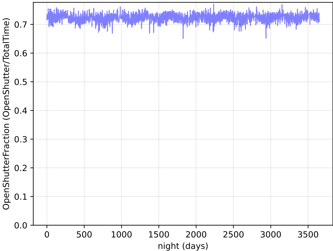
roll_pause_mjdp180_v3.4_10yrs Per night: OpenShutterFraction
