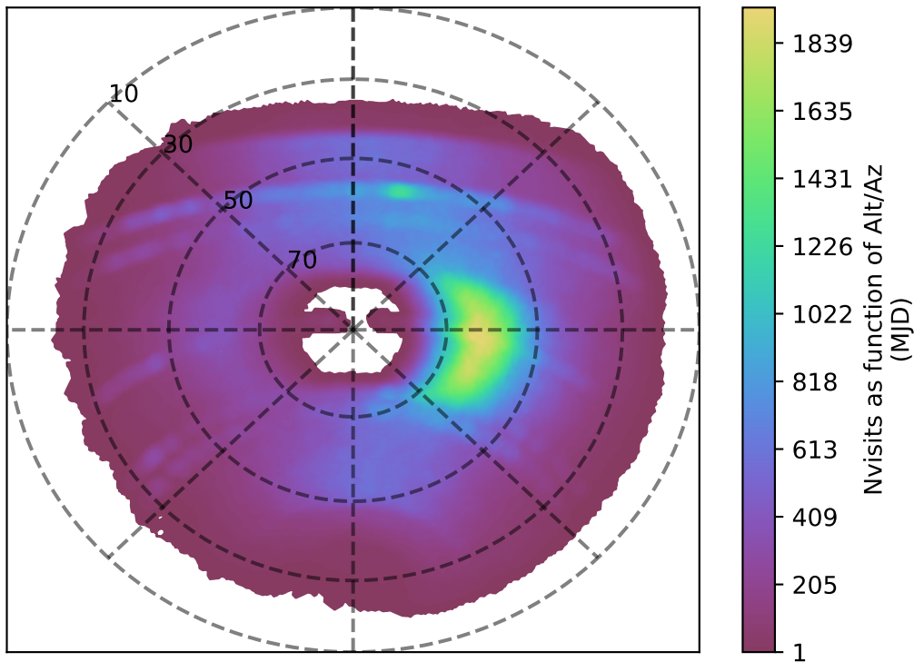
roll_pause_mjdp180_v3.4_10yrs y band: Nvisits as function of Alt/Az
