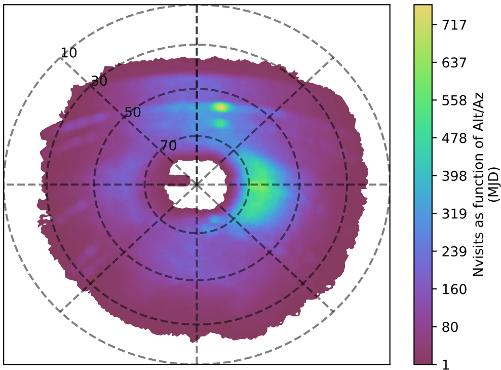
roll_pause_mjdp180_v3.4_10yrs u band: Nvisits as function of Alt/Az
