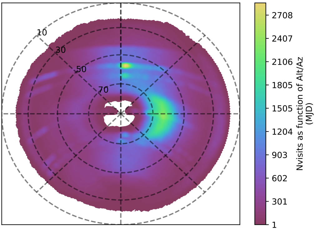
roll_pause_mjdp180_v3.4_10yrs i band: Nvisits as function of Alt/Az
