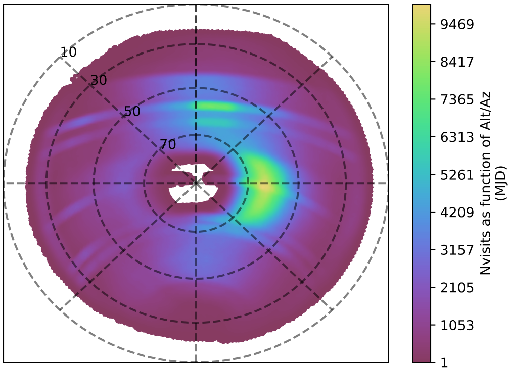
roll_pause_mjdp180_v3.4_10yrs all bands: Nvisits as function of Alt/Az
