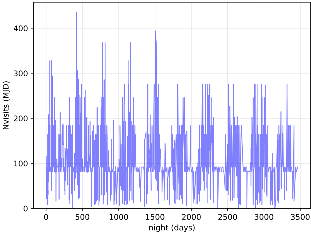
roll_pause_mjdp180_v3.4_10yrs DDF: Nvisits
