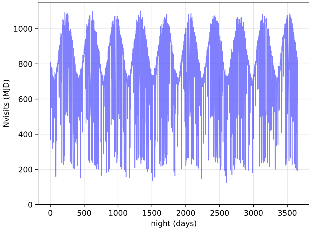
roll_pause_mjdp180_v3.4_10yrs All visits: Nvisits
