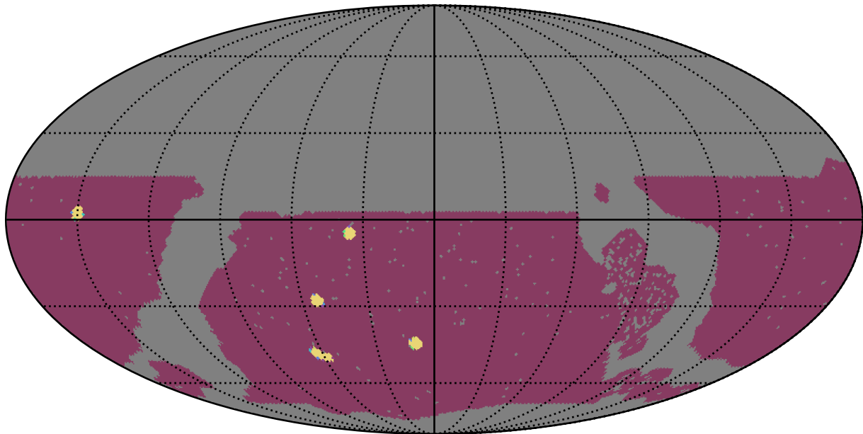
roll_pause_mjdp180_v3.4_10yrs WFD: NumberOfQuickRevisits
