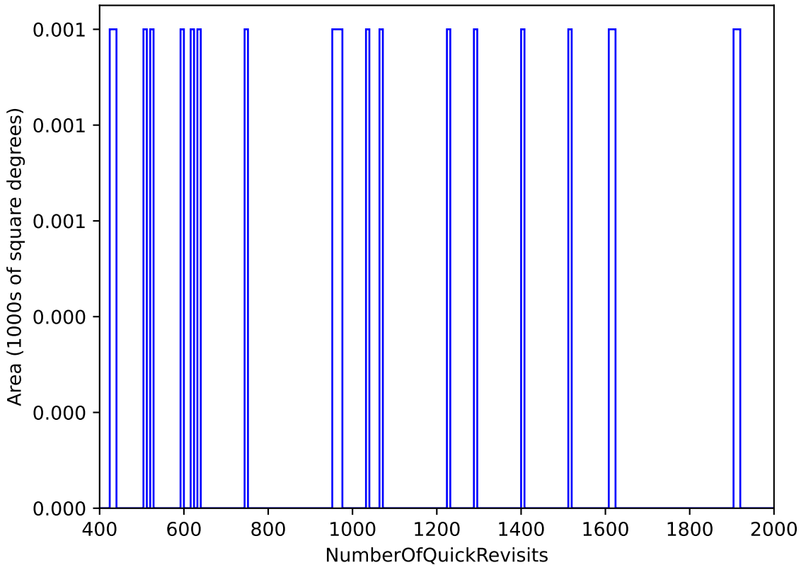
roll_pause_mjdp180_v3.4_10yrs WFD: NumberOfQuickRevisits
