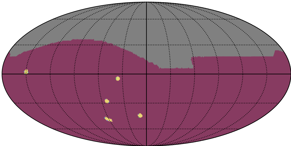
roll_pause_mjdp180_v3.4_10yrs All sky: NumberOfQuickRevisits
