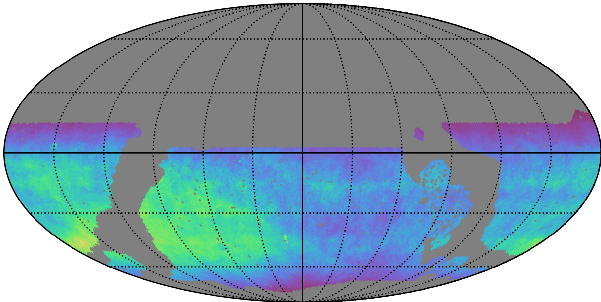
roll_pause_mjdp180_v3.4_10yrs WFD z band: Normalized Teff
