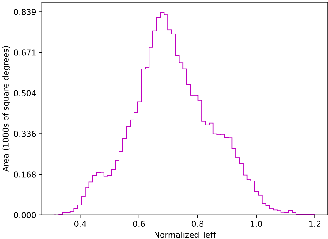
roll_pause_mjdp180_v3.4_10yrs WFD z band: Normalized Teff
