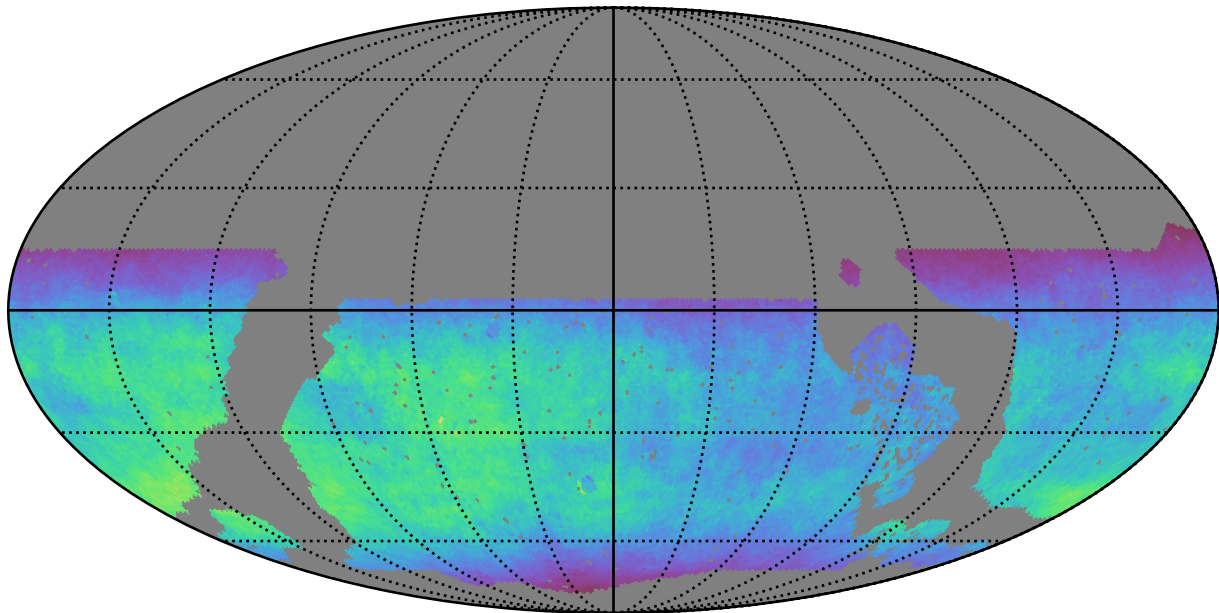
roll_pause_mjdp180_v3.4_10yrs WFD y band: Normalized Teff
