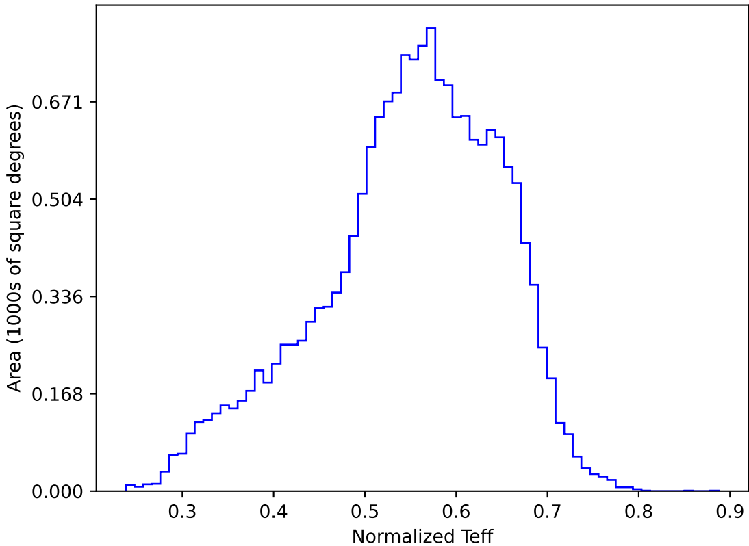
roll_pause_mjdp180_v3.4_10yrs WFD y band: Normalized Teff
