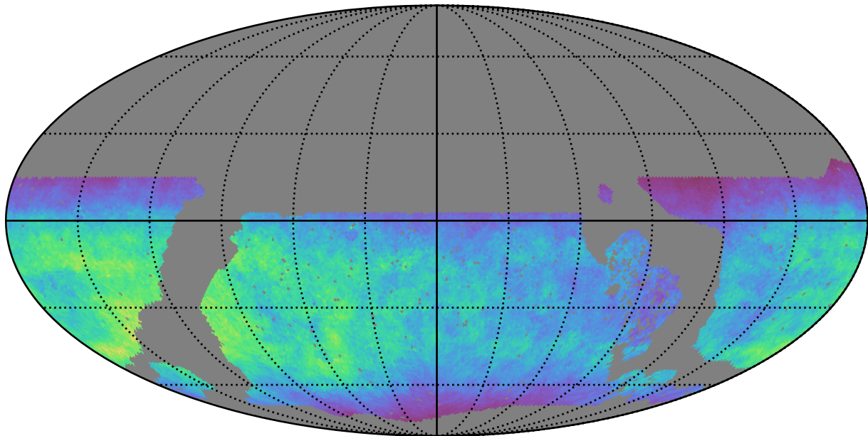
roll_pause_mjdp180_v3.4_10yrs WFD u band: Normalized Teff
