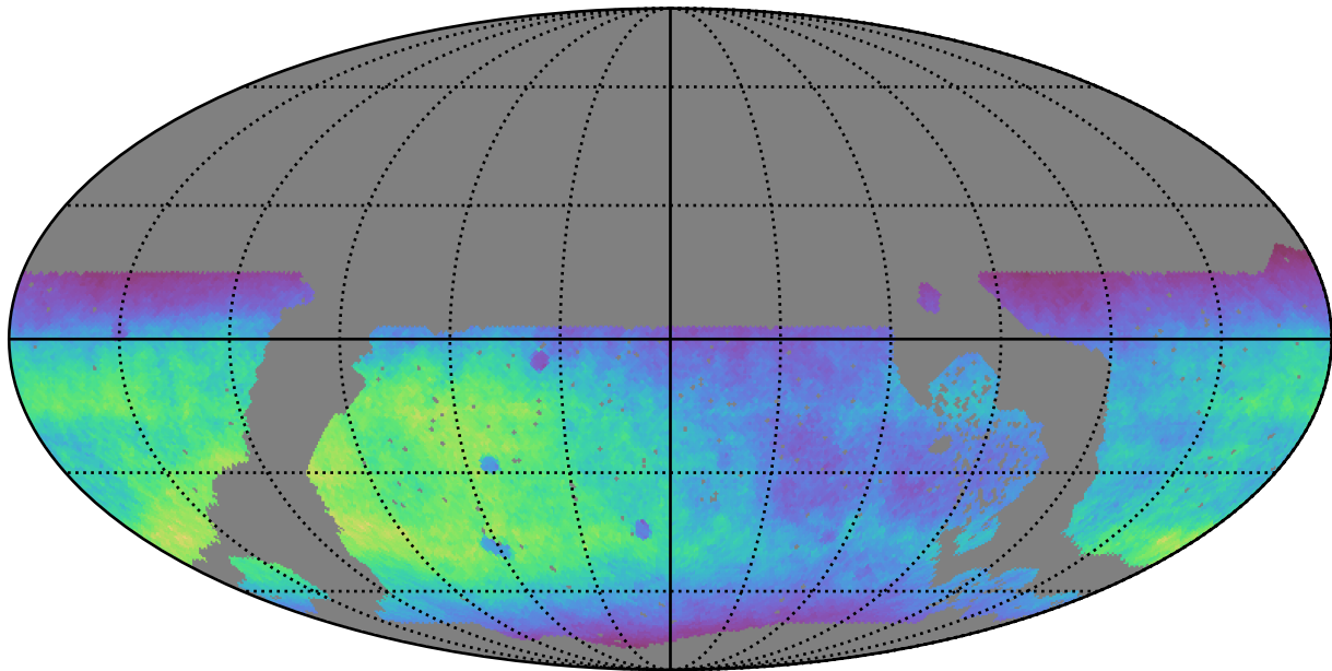
roll_pause_mjdp180_v3.4_10yrs WFD r band: Normalized Teff
