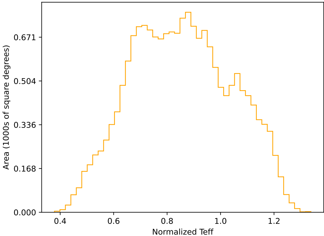
roll_pause_mjdp180_v3.4_10yrs WFD r band: Normalized Teff
