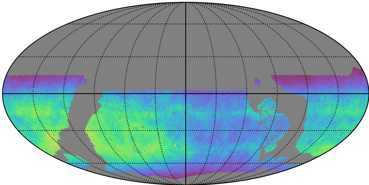
roll_pause_mjdp180_v3.4_10yrs WFD i band: Normalized Teff
