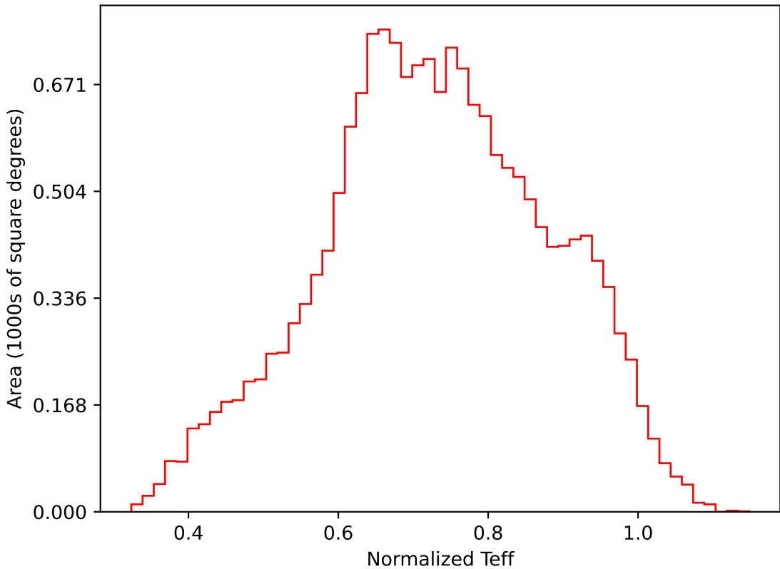
roll_pause_mjdp180_v3.4_10yrs WFD i band: Normalized Teff
