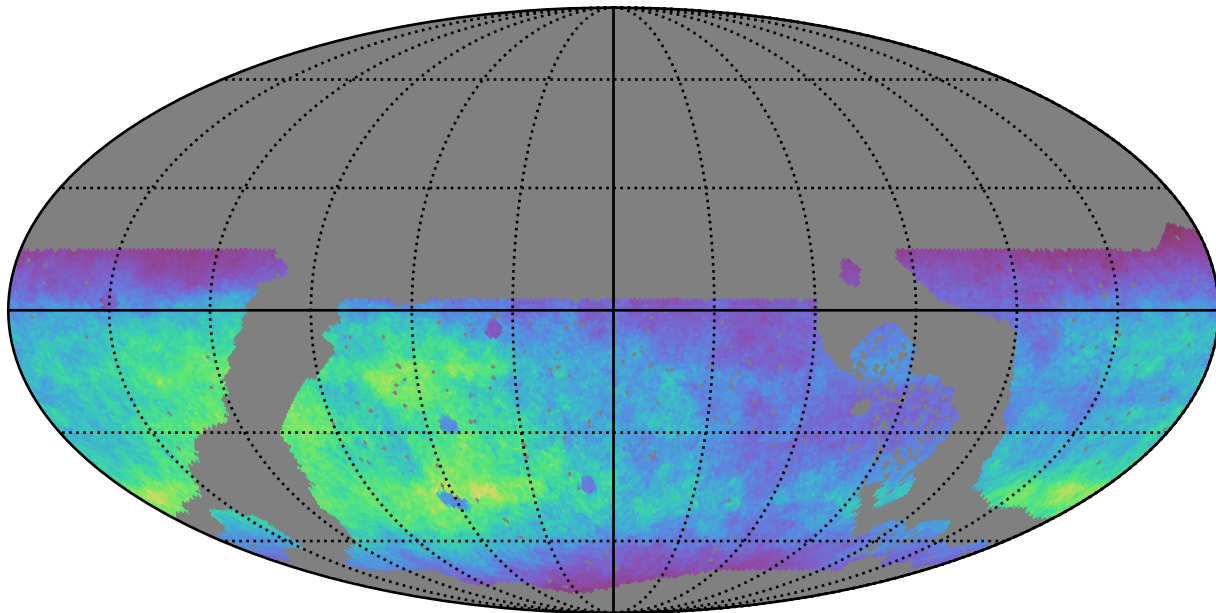
roll_pause_mjdp180_v3.4_10yrs WFD g band: Normalized Teff
